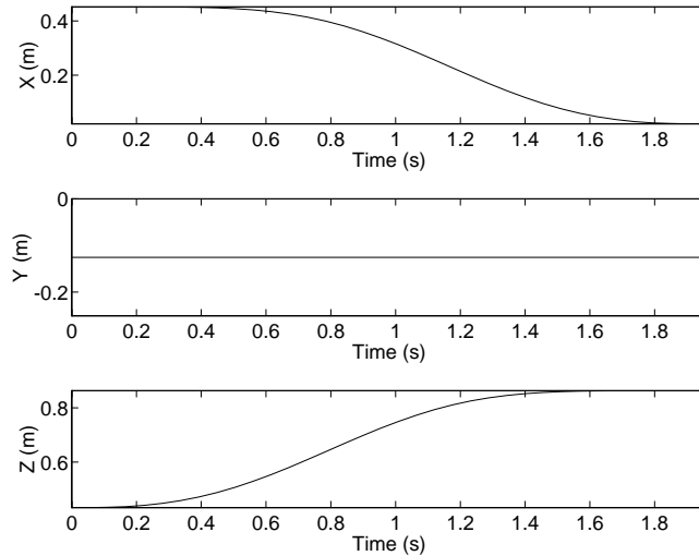
Figure 3: Cartesian coordinates of wrist for the trajectory of Figure 2.
